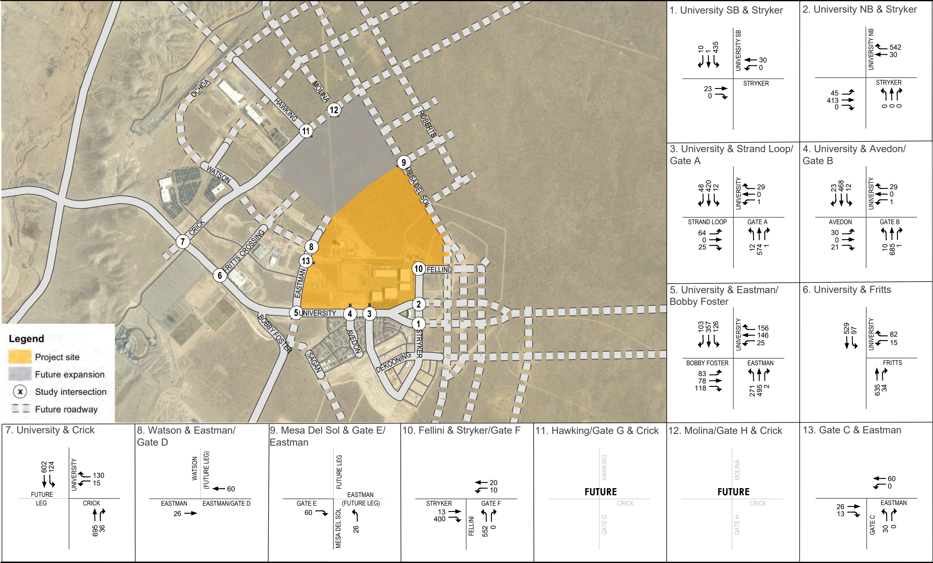
Figure 12 Implementation Year (2026) With Project PM Peak Hour Volumes 22
